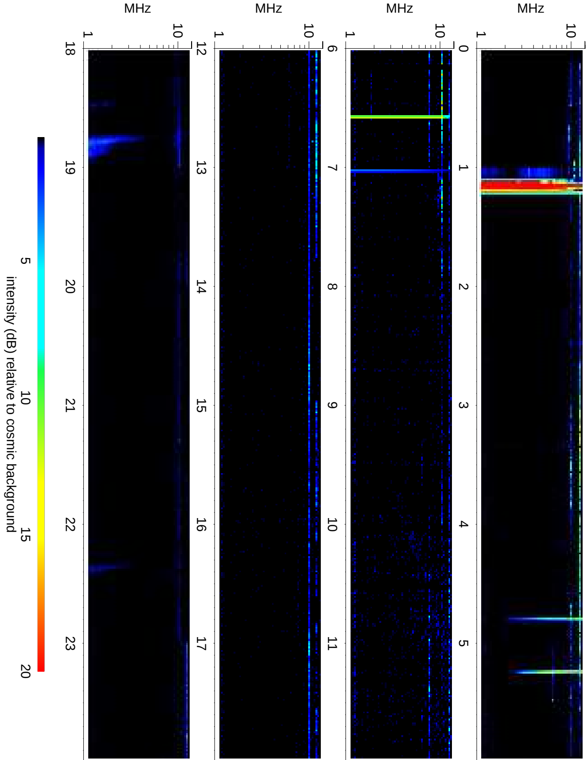
Wind Waves RAD2 receiver: 2008/01/30
