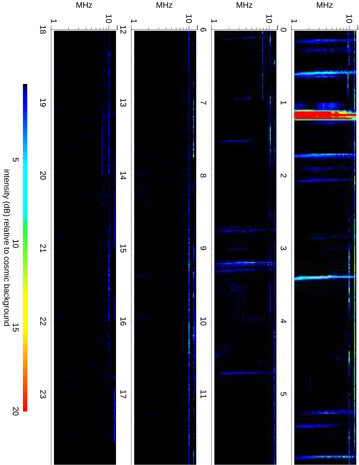
Wind Waves RAD2 receiver: 2008/02/03
