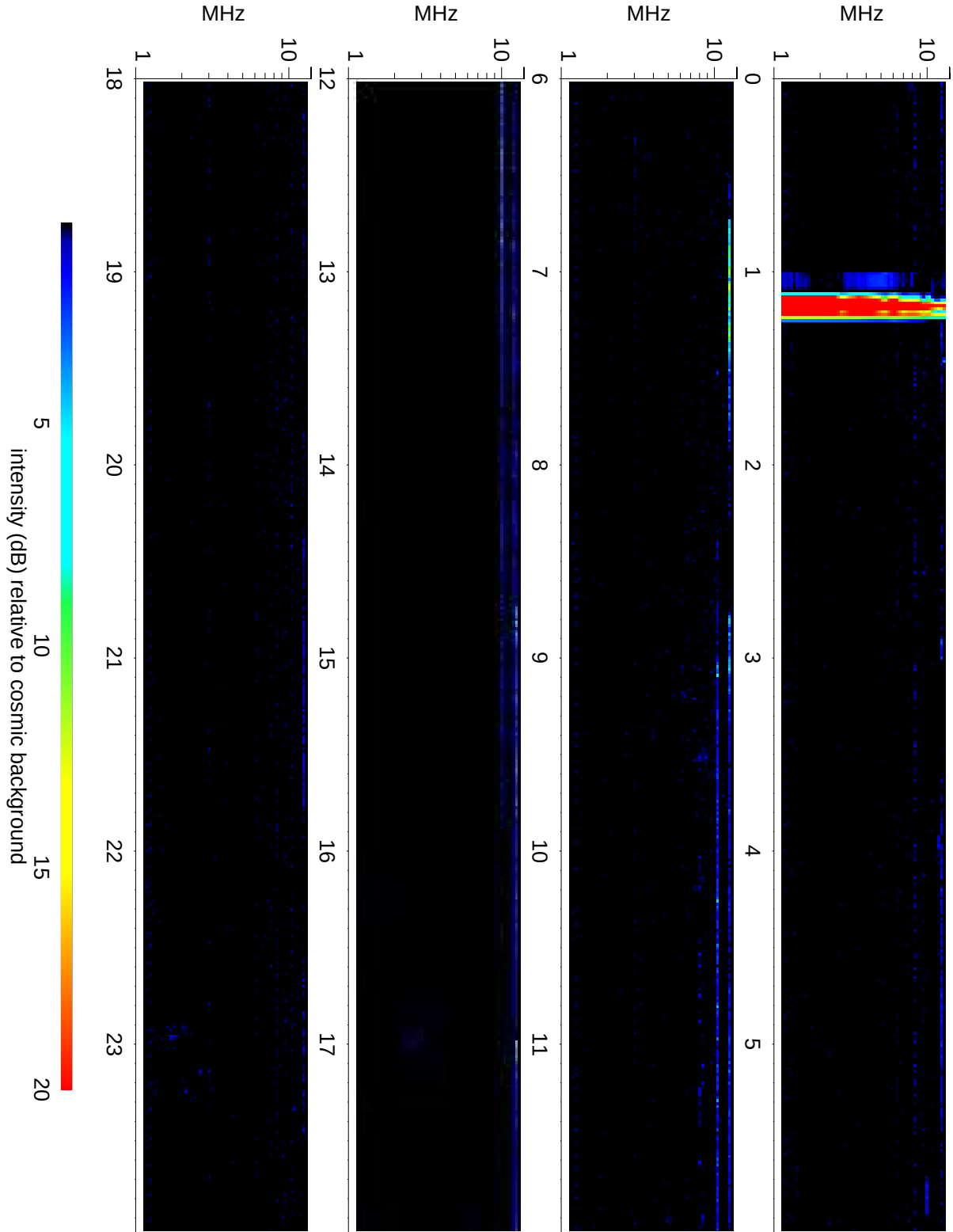
Wind Waves RAD2 receiver: 2008/04/01
