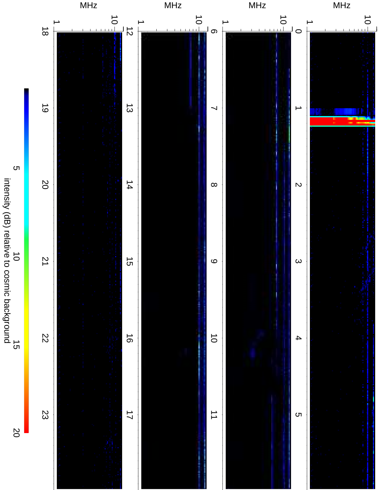
Wind Waves RAD2 receiver: 2008/04/19
