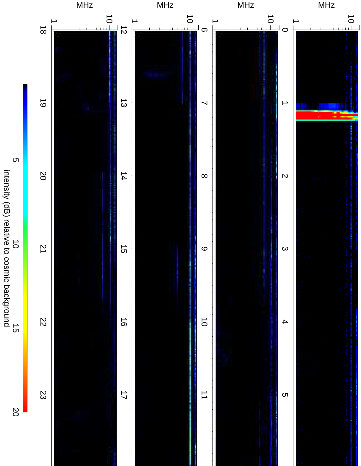
Wind Waves RAD2 receiver: 2008/05/05
