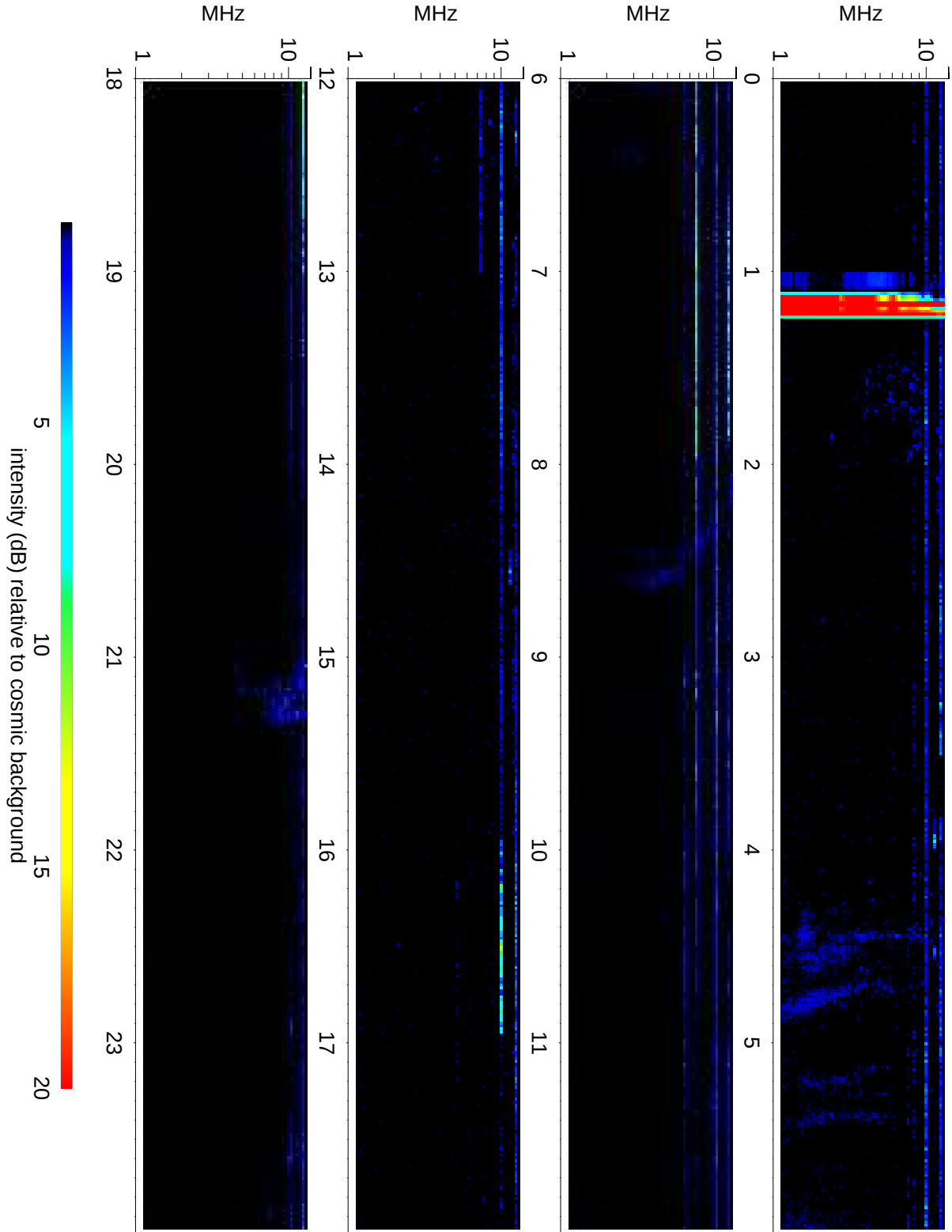
Wind Waves RAD2 receiver: 2008/06/04
