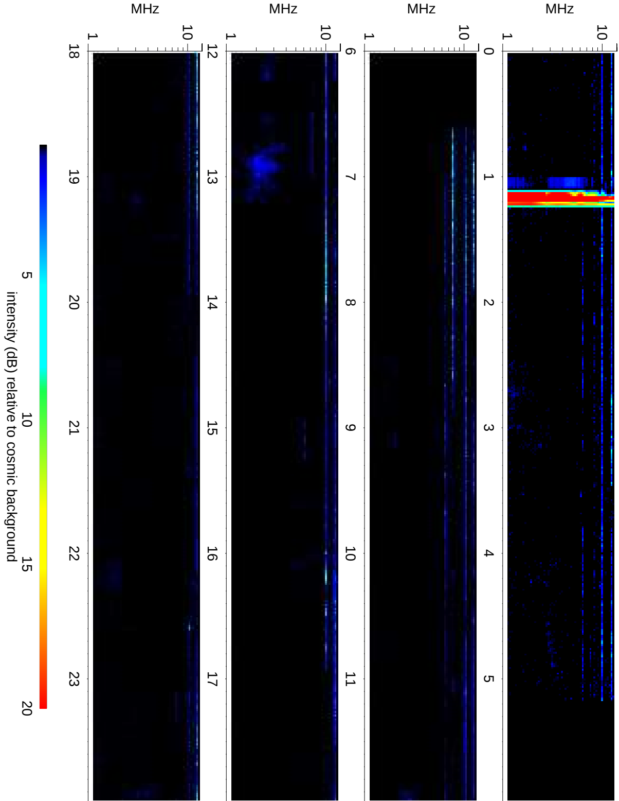
Wind Waves RAD2 receiver: 2008/06/10
