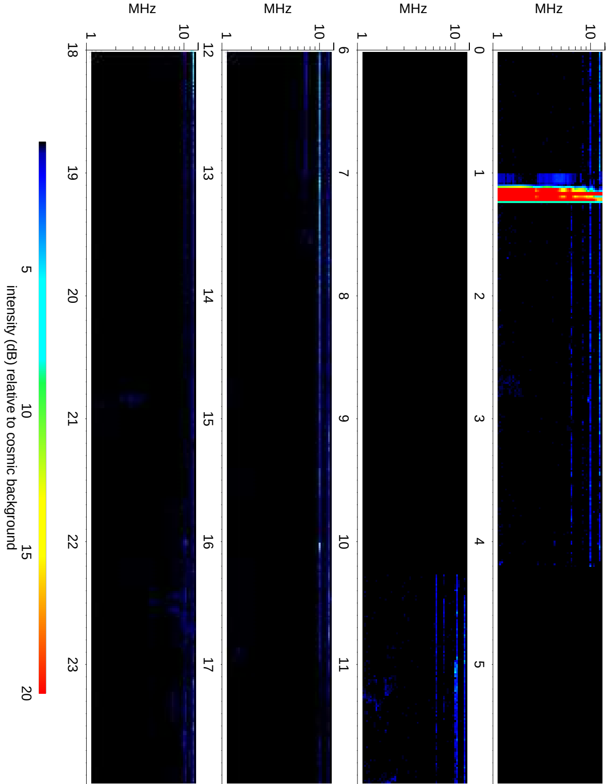
Wind Waves RAD2 receiver: 2008/06/12
