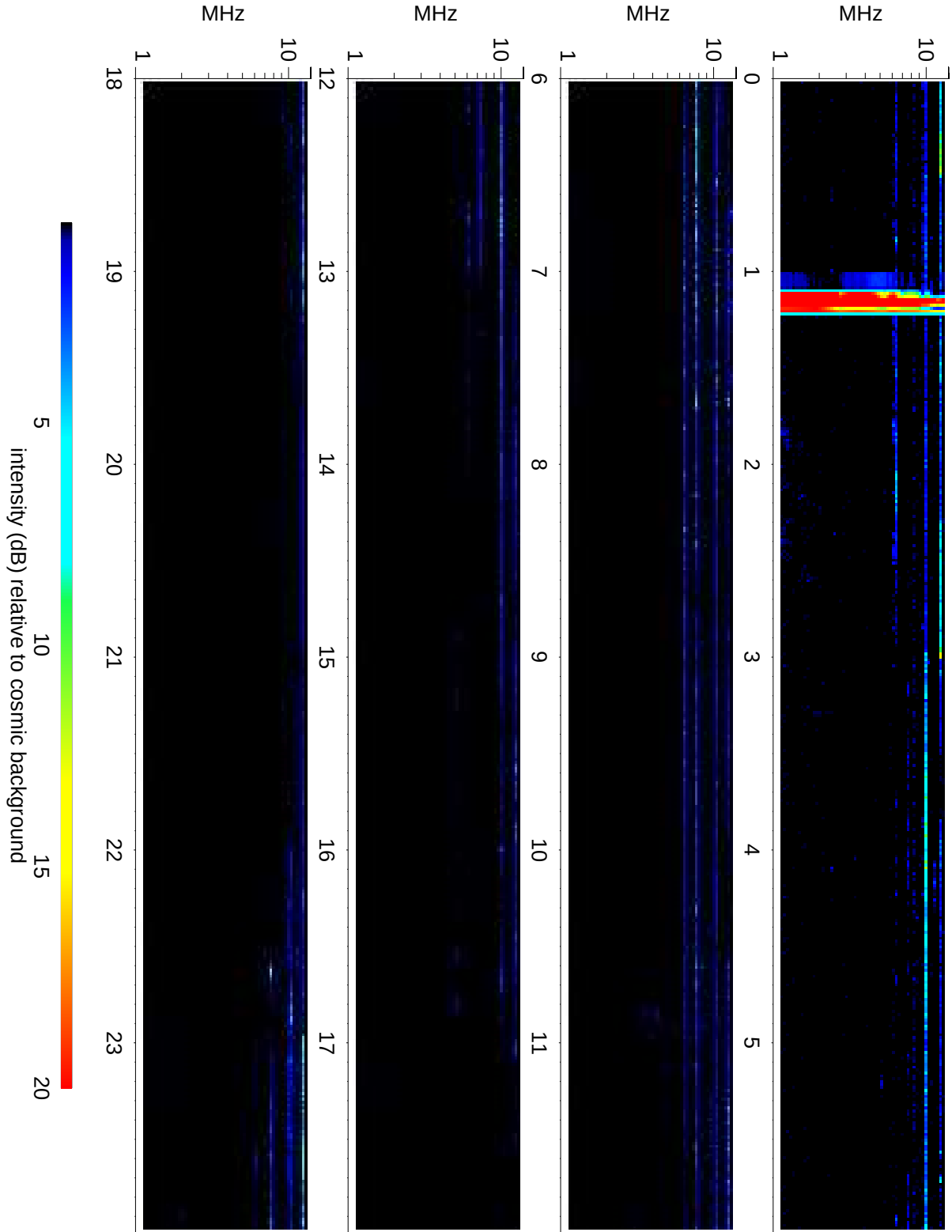
Wind Waves RAD2 receiver: 2008/07/08
