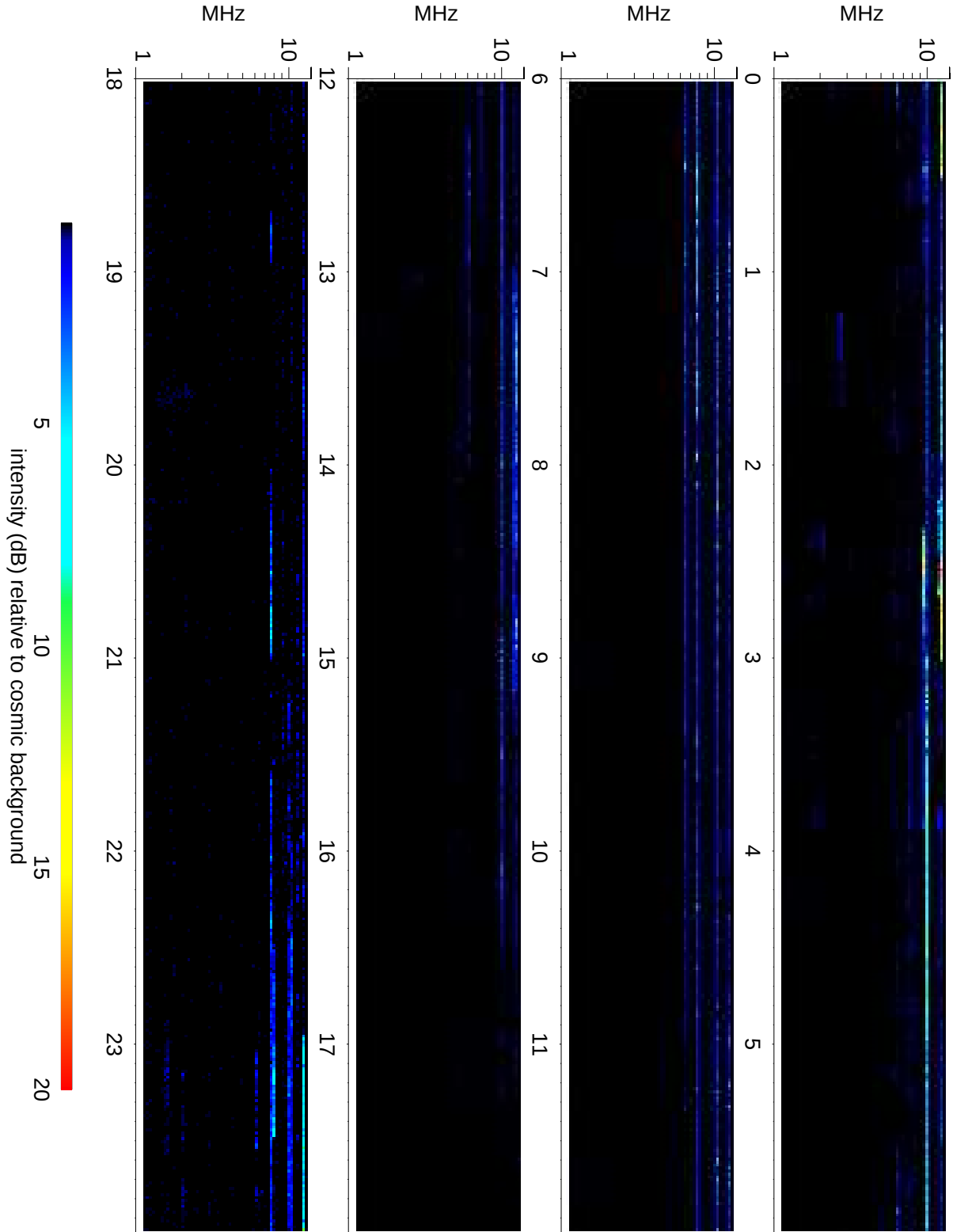
Wind Waves RAD2 receiver: 2008/08/04
