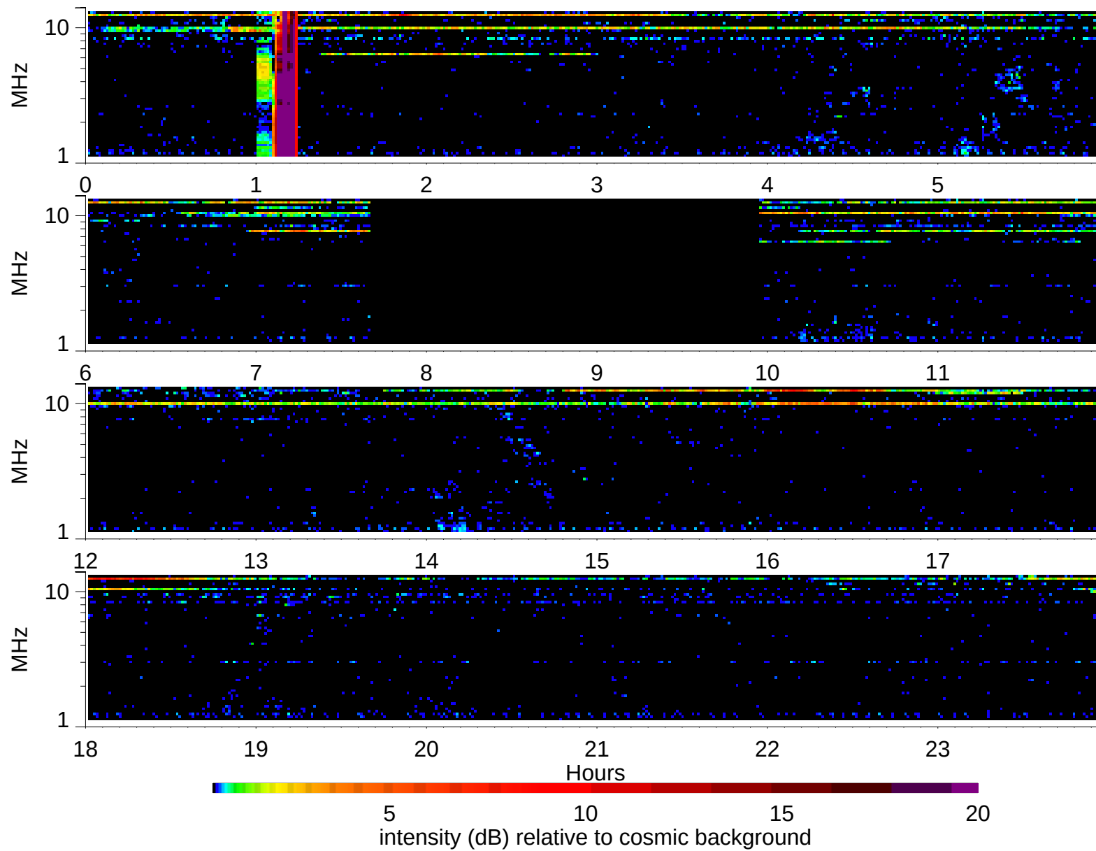
Wind Waves RAD2 receiver: 2008/9/4
