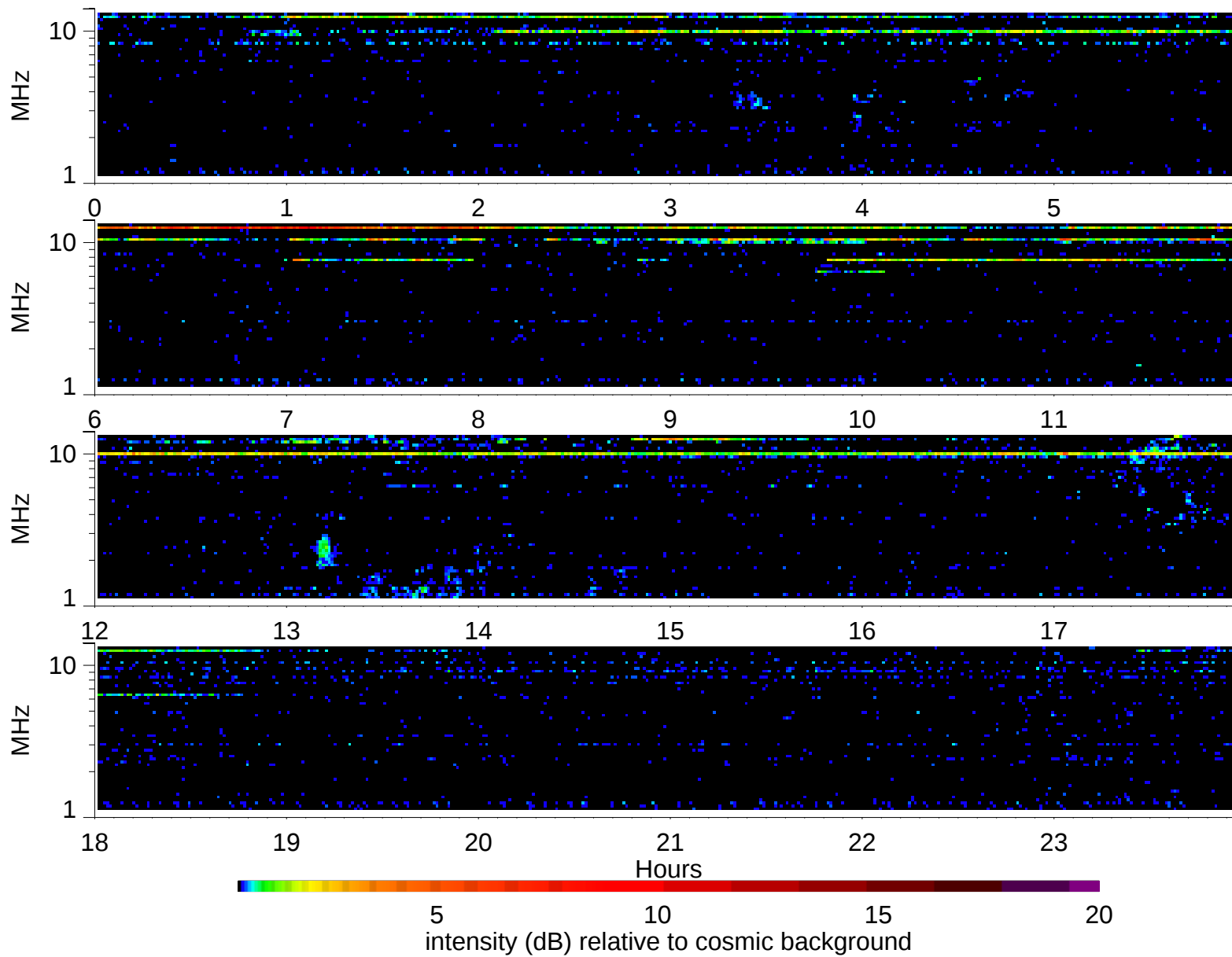
Wind Waves RAD2 receiver: 2008/9/21
