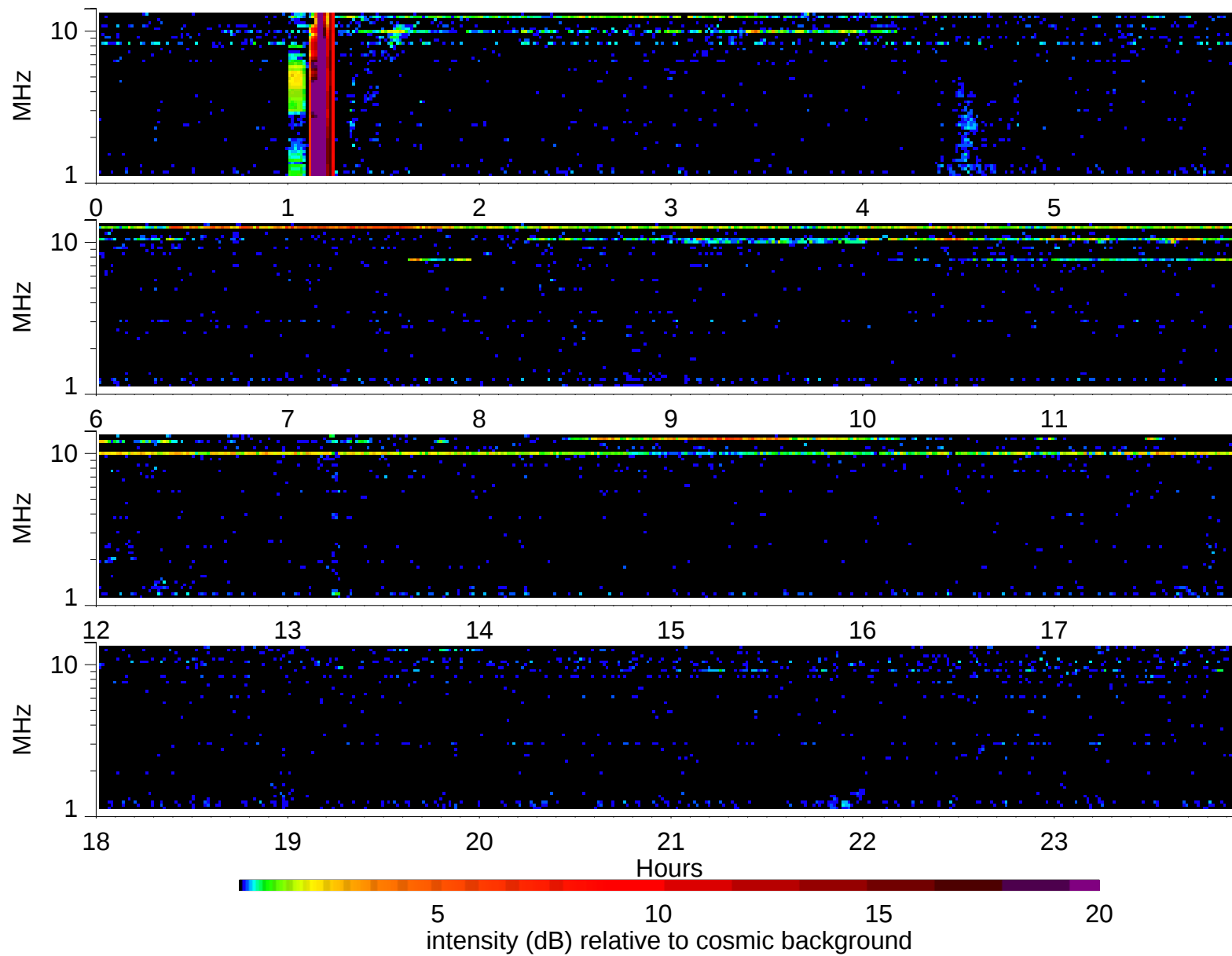
Wind Waves RAD2 receiver: 2008/9/26
