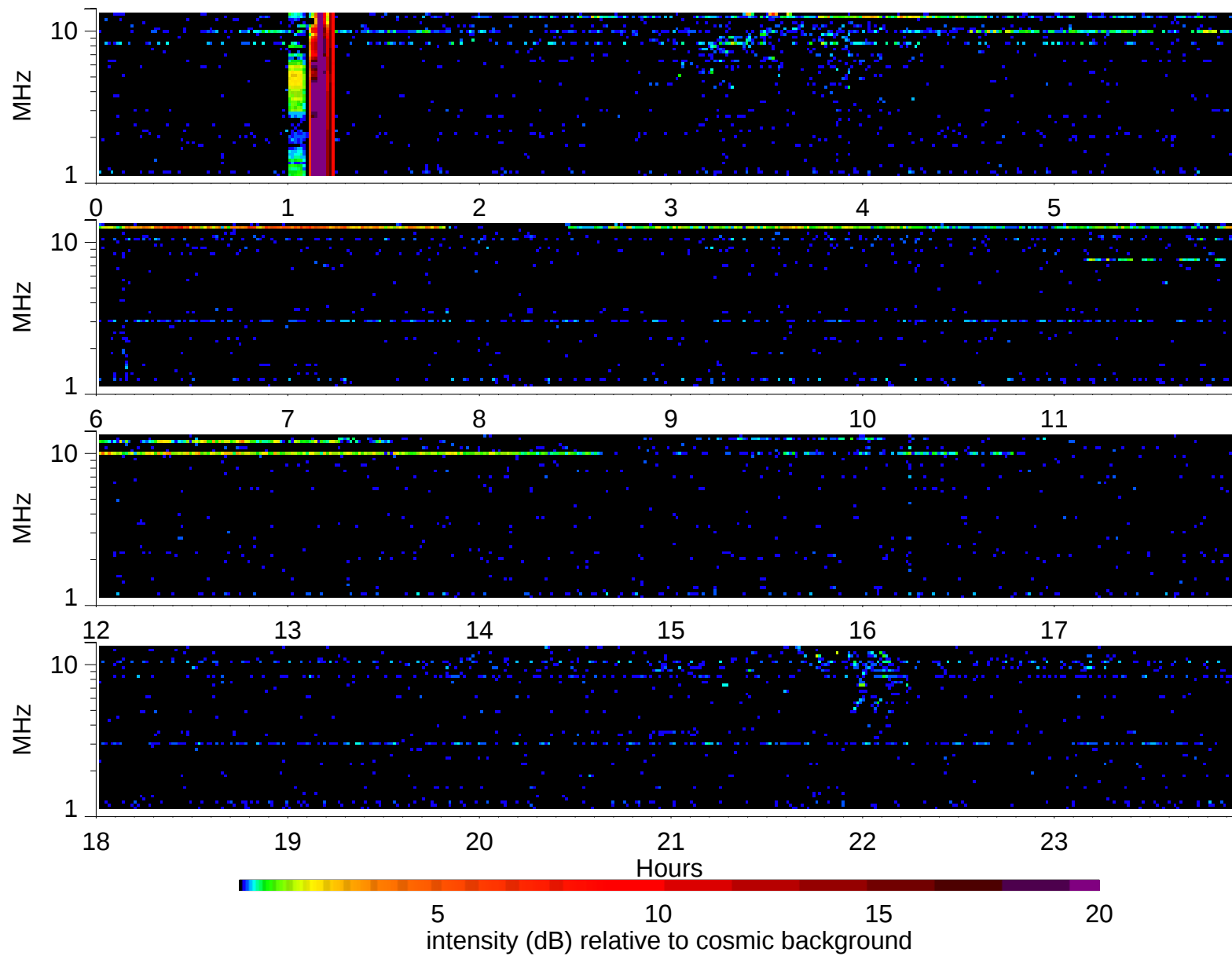
Wind Waves RAD2 receiver: 2008/10/4
