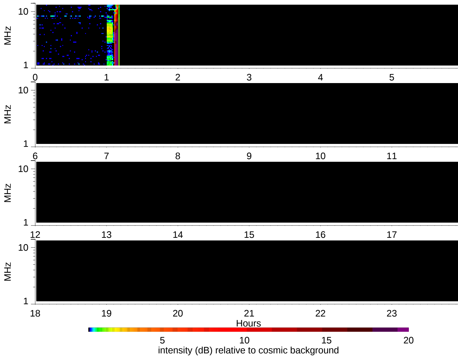
Wind Waves RAD2 receiver: 2008/10/10
