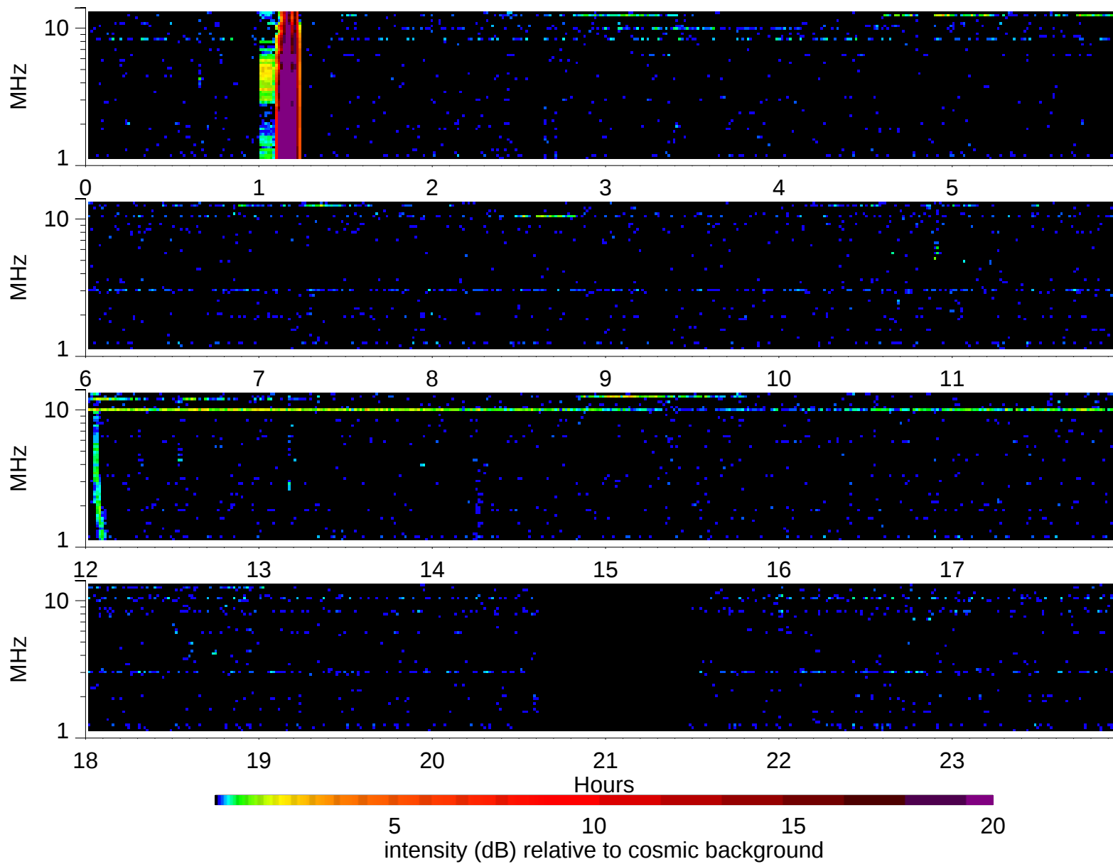
Wind Waves RAD2 receiver: 2008/10/14
