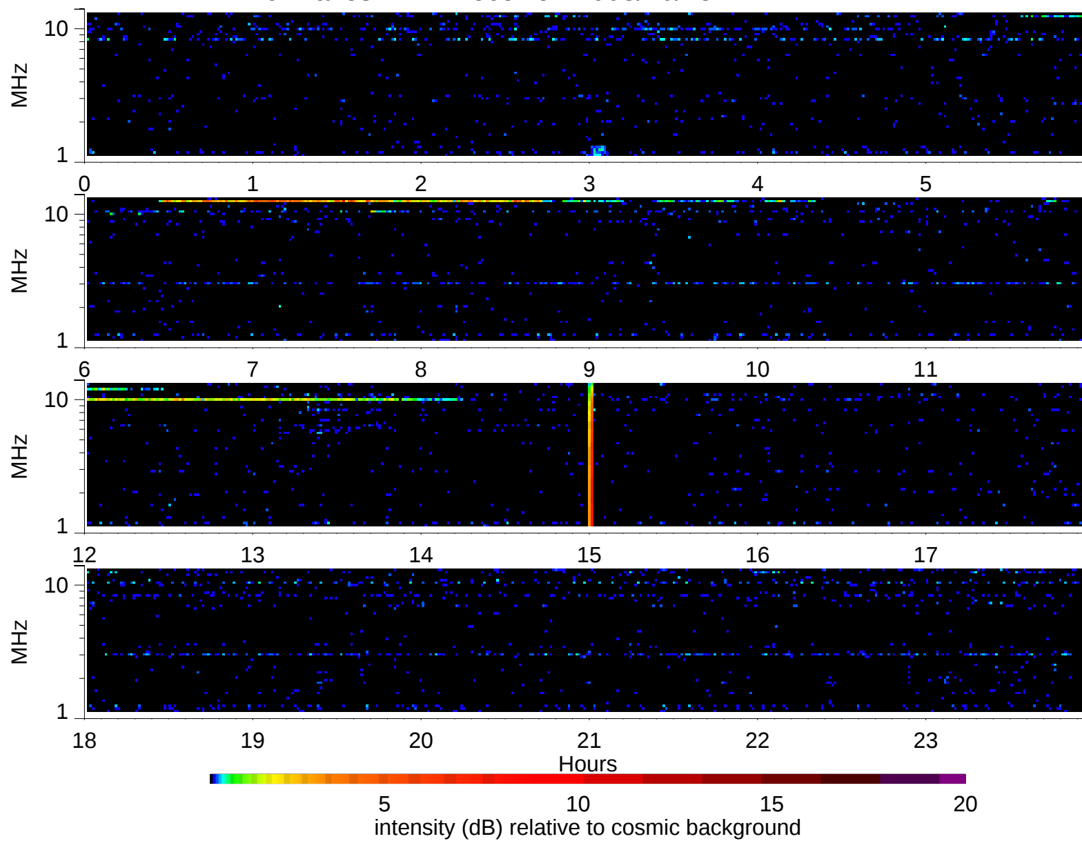
Wind Waves RAD2 receiver: 2008/10/15
