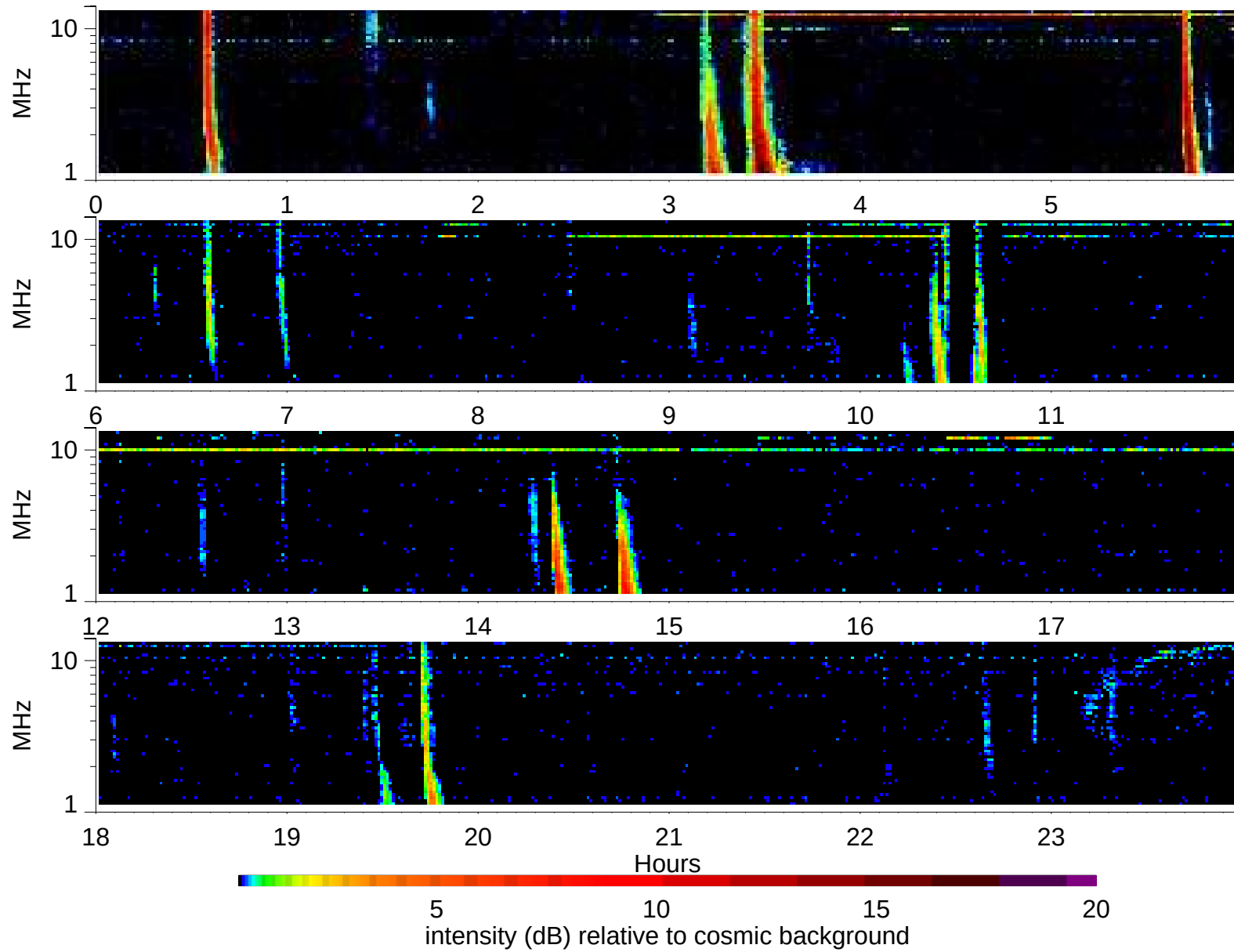
Wind Waves RAD2 receiver: 2008/11/04
