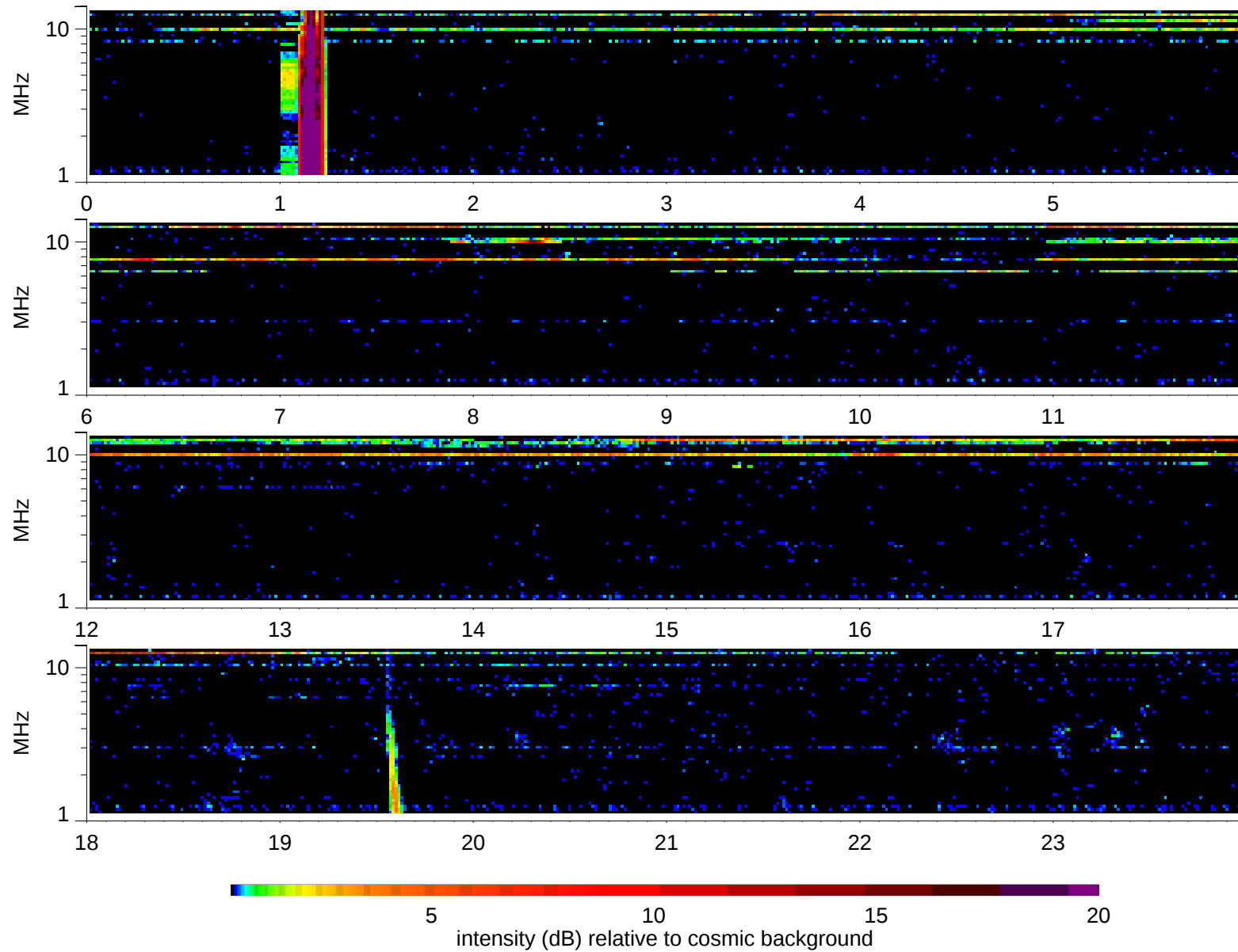
Wind Waves RAD2 receiver: 2009/05/02
