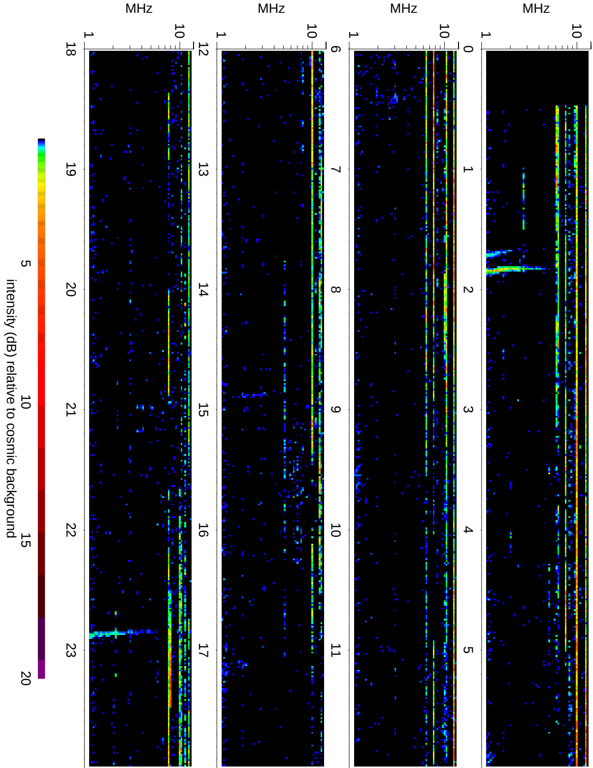
Wind Waves RAD2 receiver: 2009/07/18
