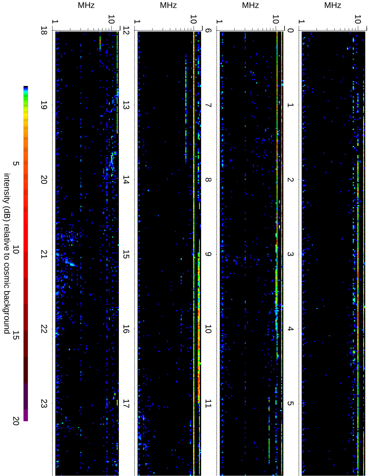
Wind Waves RAD2 receiver: 2009/09/14
