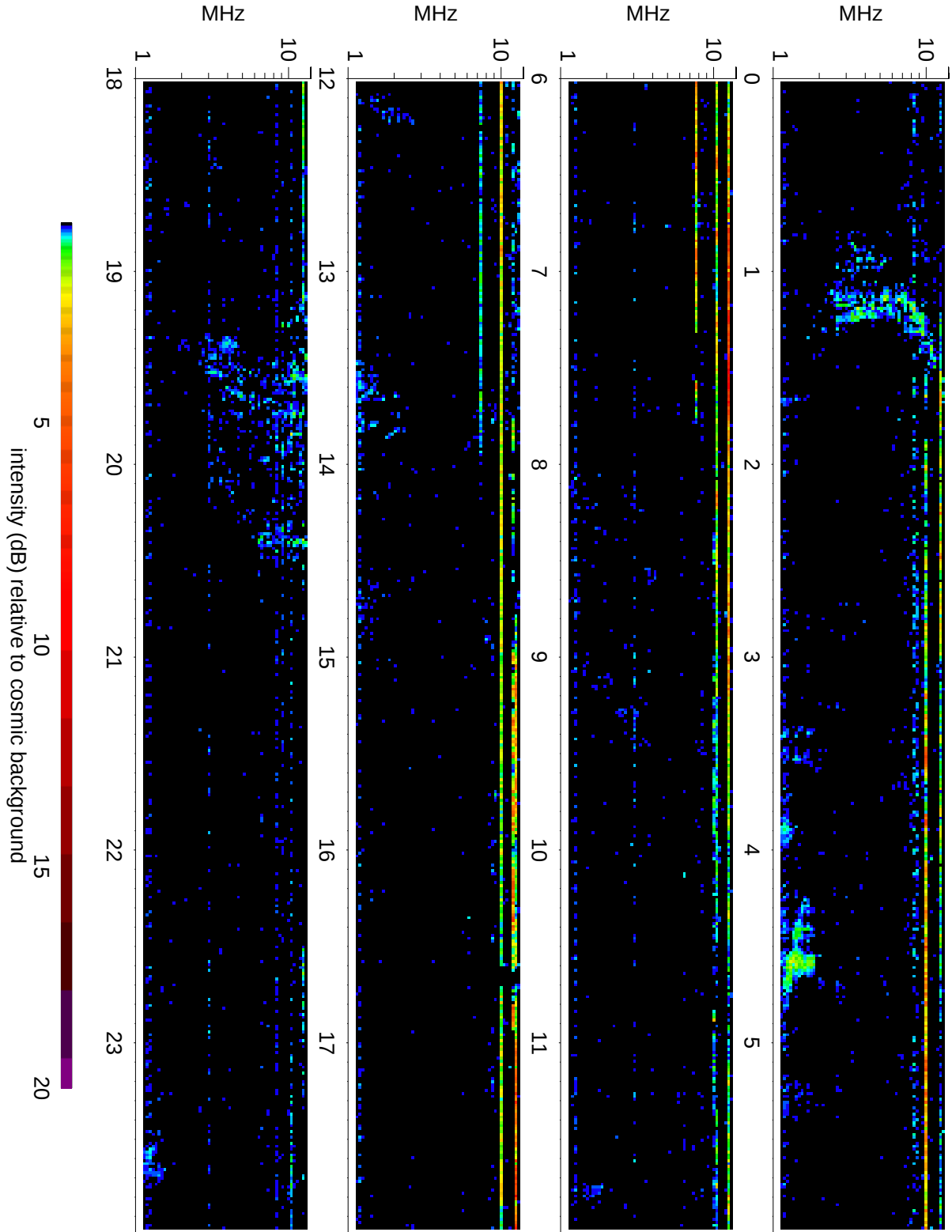
Wind Waves RAD2 receiver: 2009/09/16
