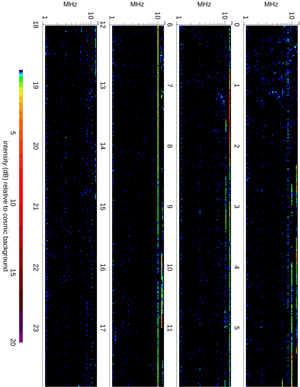
Wind Waves RAD2 receiver: 2009/10/08
