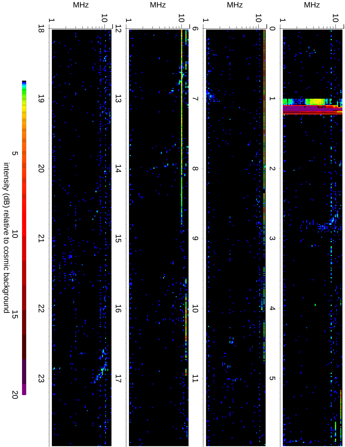
Wind Waves RAD2 receiver: 2009/10/19
