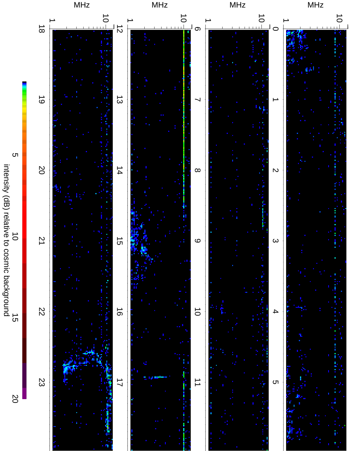
Wind Waves RAD2 receiver: 2009/10/24
