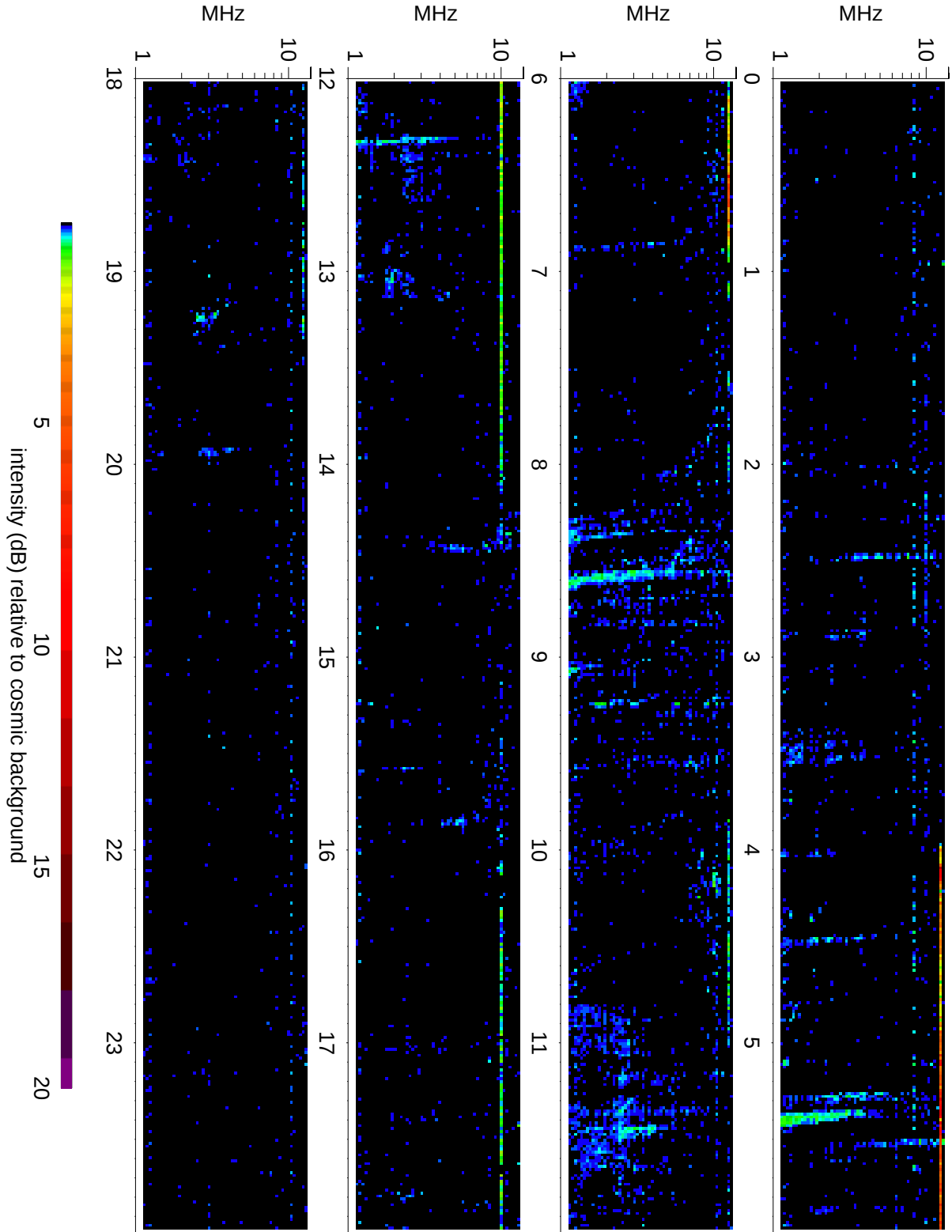
Wind Waves RAD2 receiver: 2009/10/28
