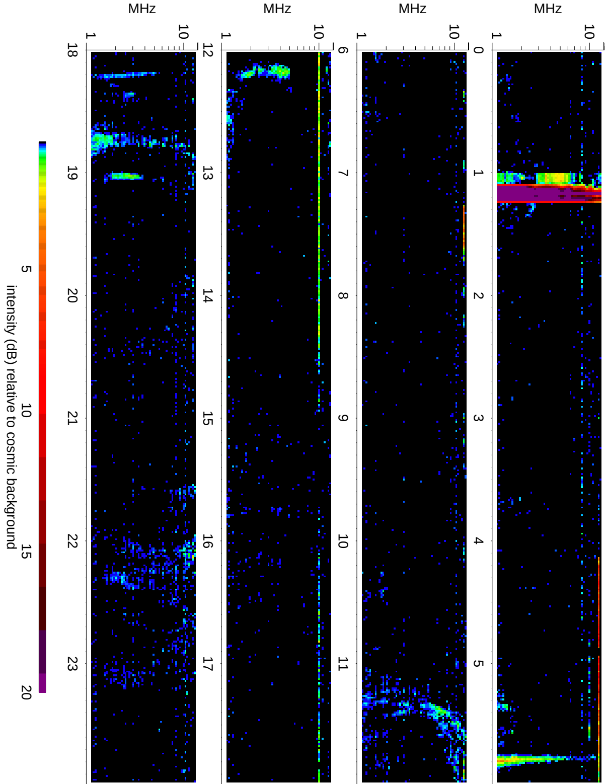
Wind Waves RAD2 receiver: 2009/10/31
