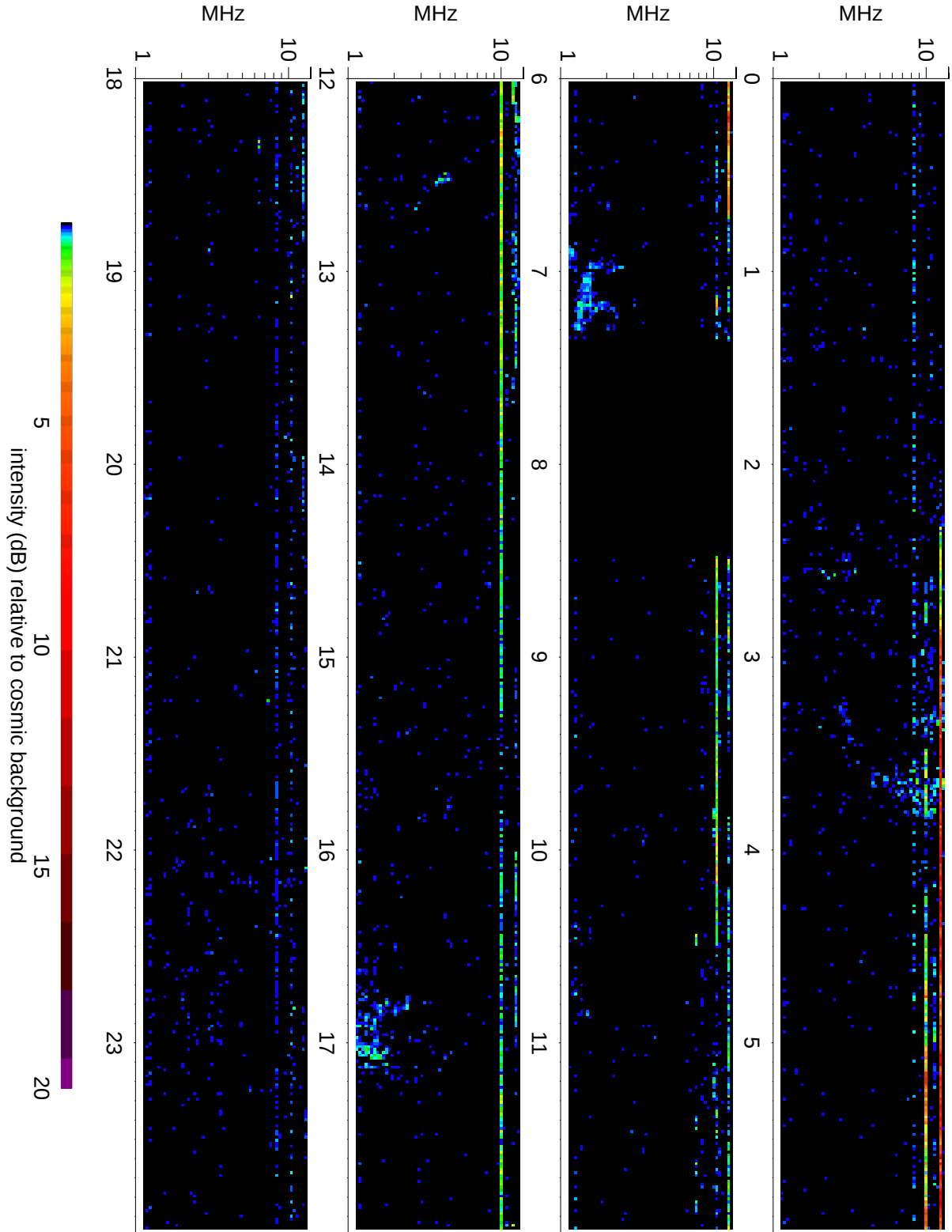
Wind Waves RAD2 receiver: 2009/11/07
