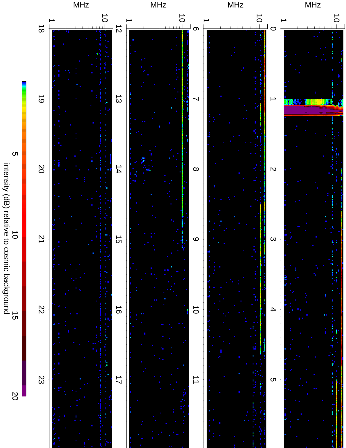
Wind Waves RAD2 receiver: 2009/11/16
