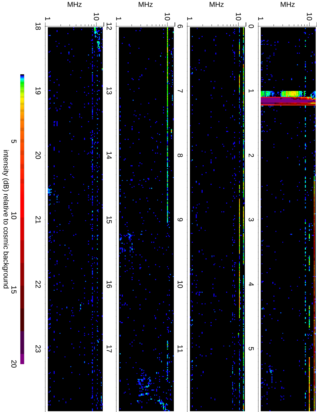
Wind Waves RAD2 receiver: 2009/11/18
