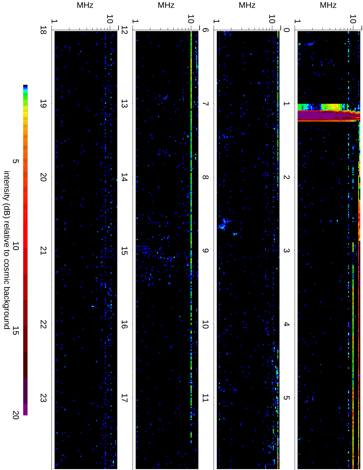
Wind Waves RAD2 receiver: 2009/11/24
