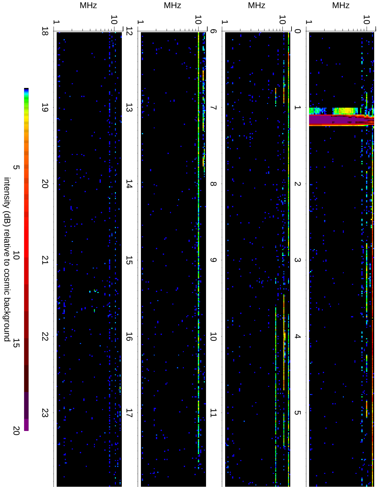
Wind Waves RAD2 receiver: 2009/12/02
