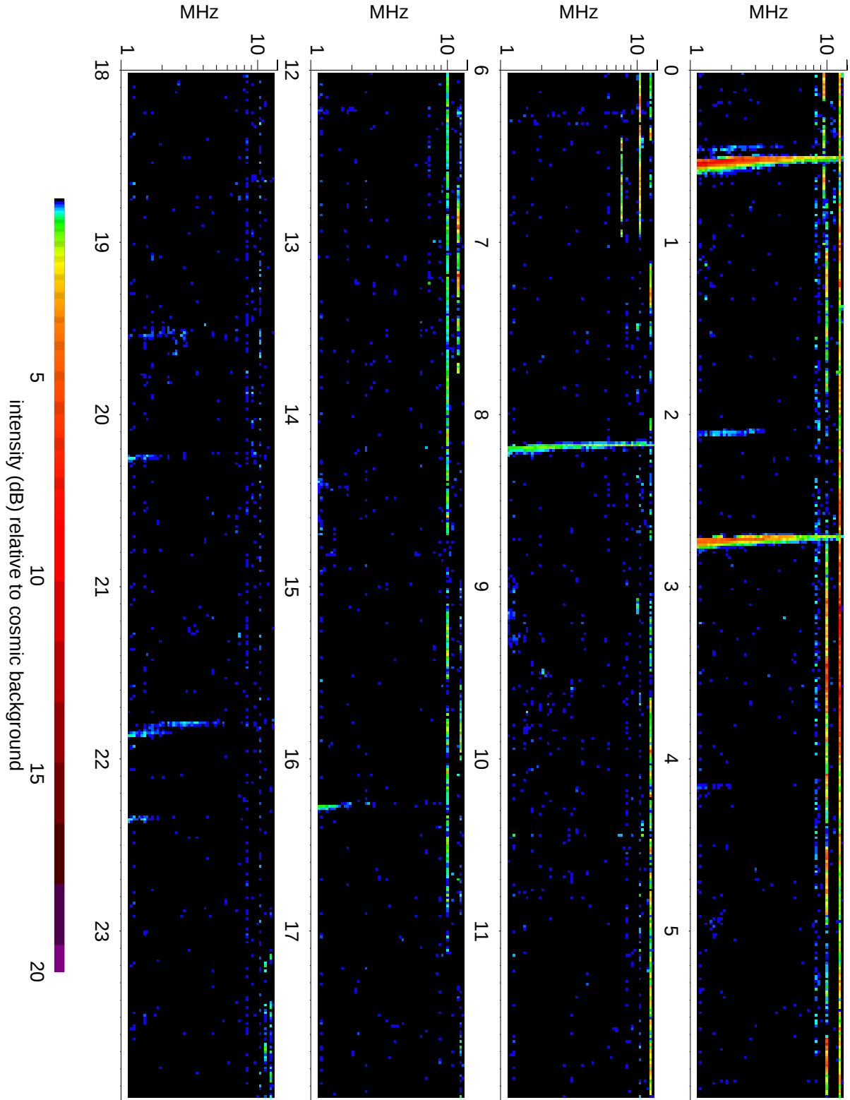
Wind Waves RAD2 receiver: 2009/12/23
