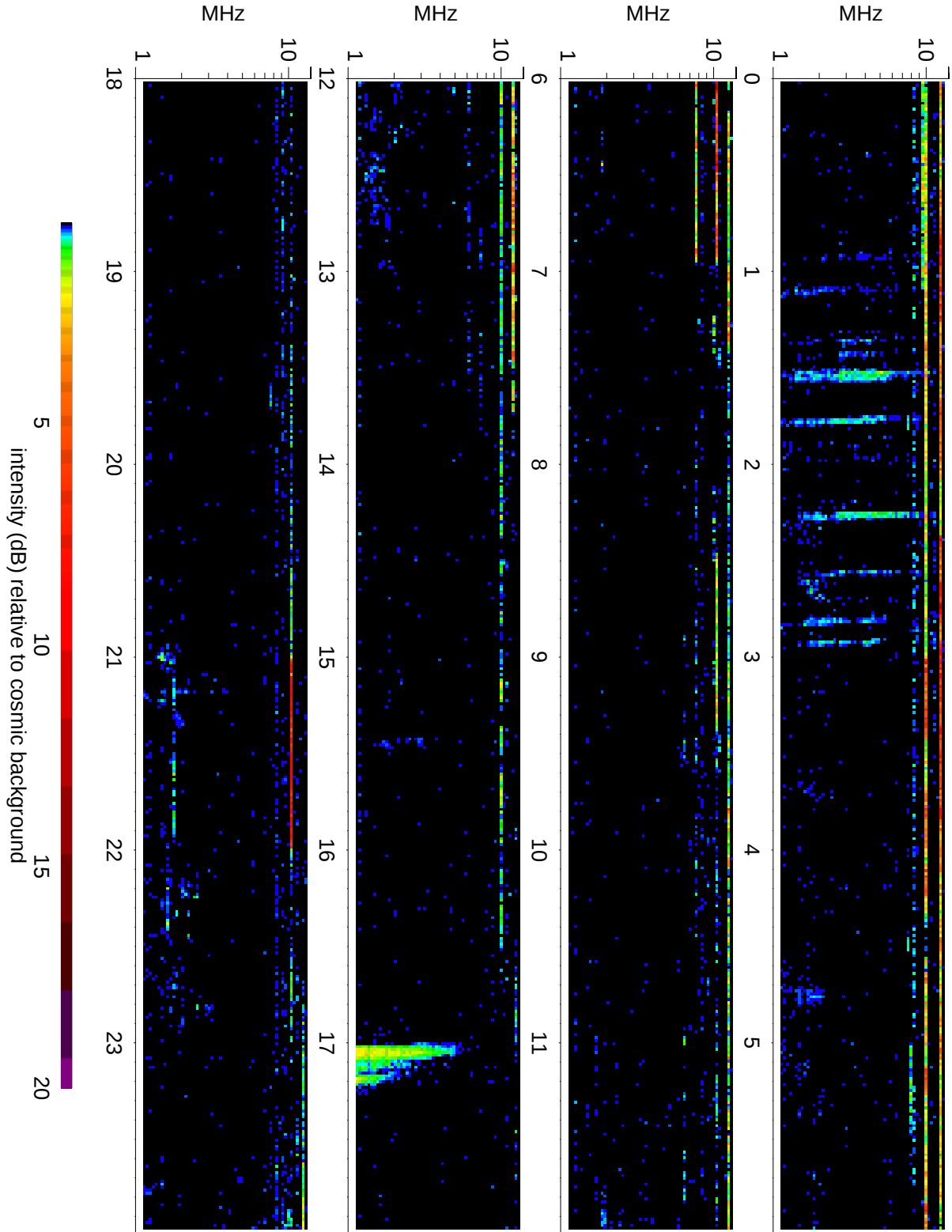
Wind Waves RAD2 receiver: 2010/01/01
