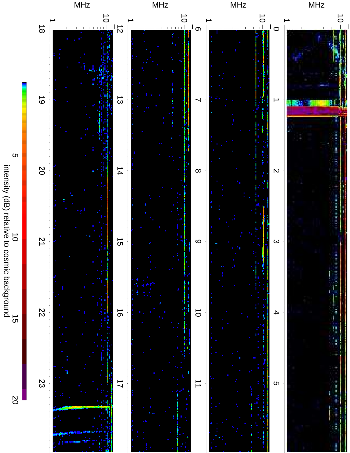
Wind Waves RAD2 receiver: 2010/01/02
