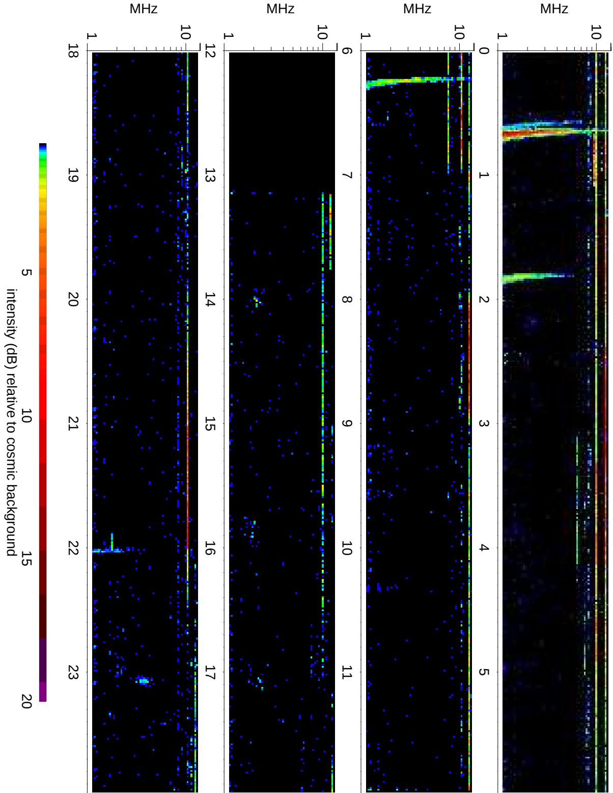
Wind Waves RAD2 receiver: 2010/01/03
