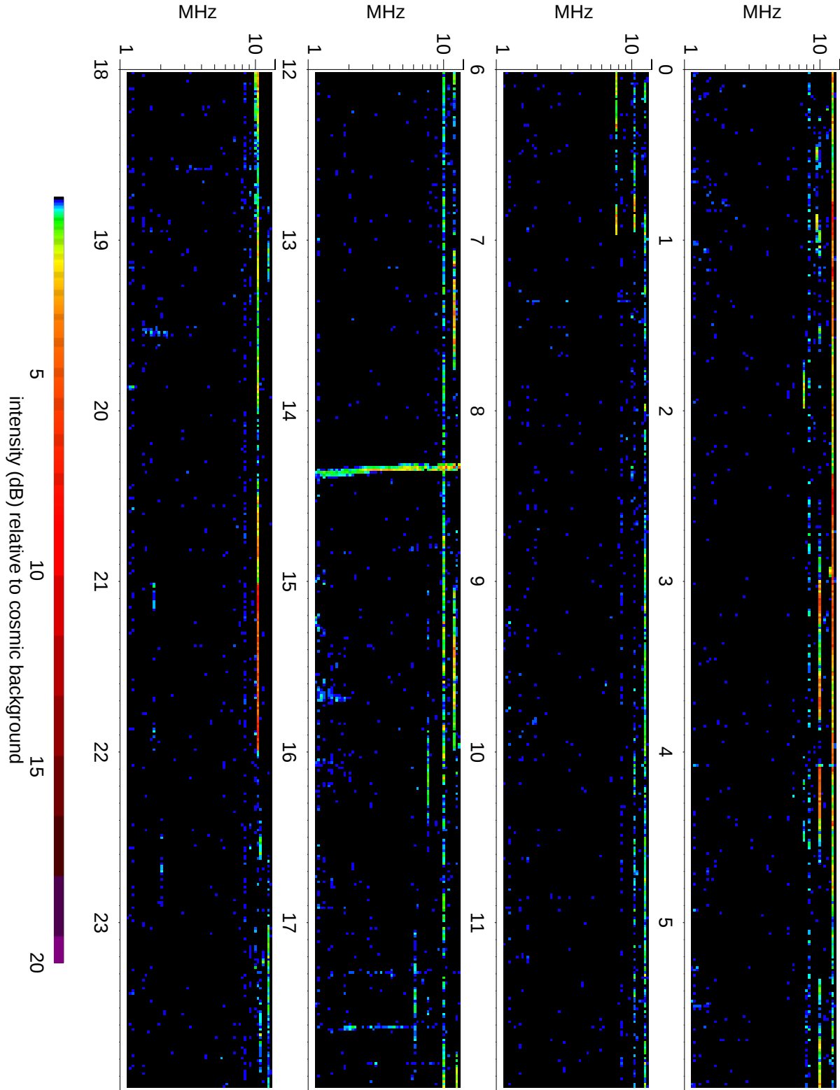
Wind Waves RAD2 receiver: 2010/01/11
