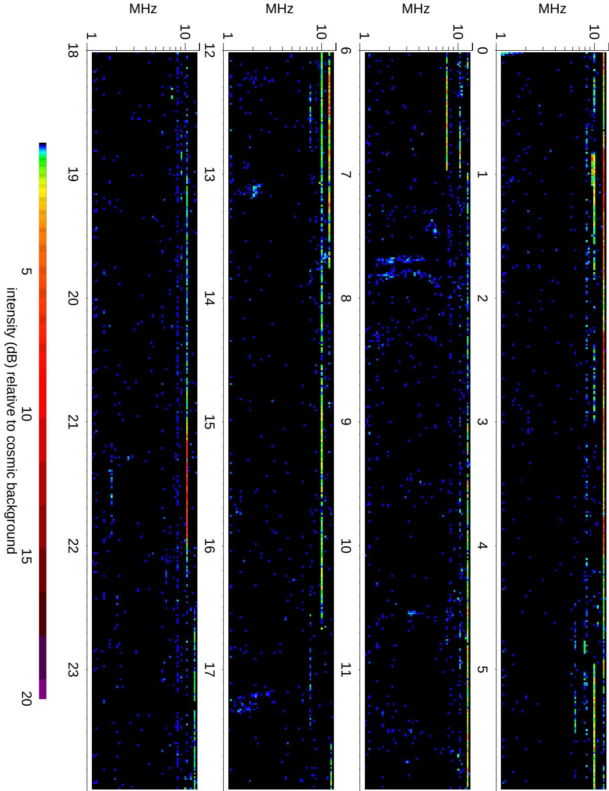
Wind Waves RAD2 receiver: 2010/01/19
