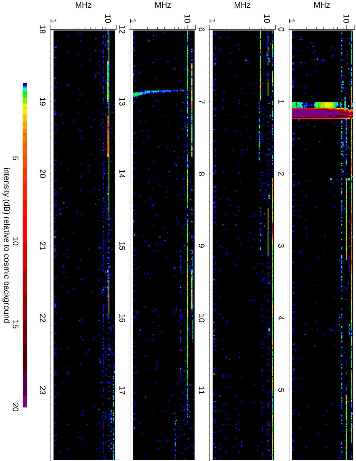
Wind Waves RAD2 receiver: 2010/01/24
