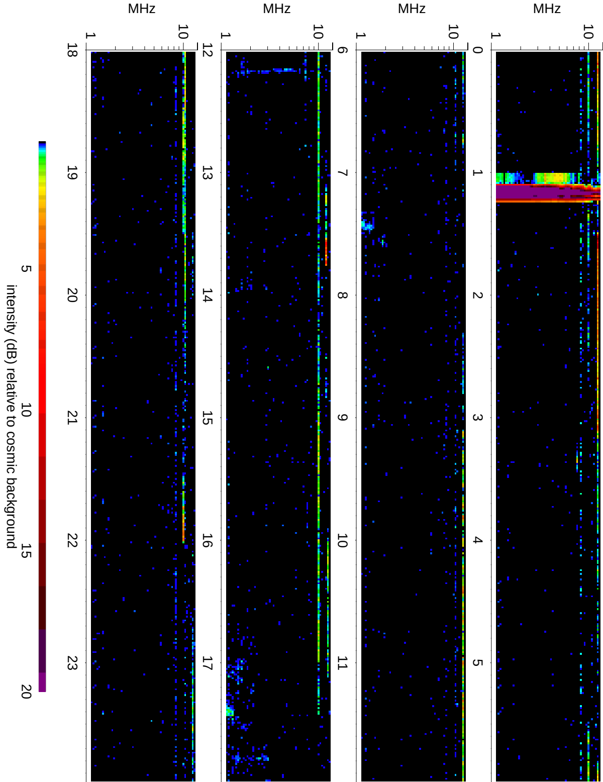
Wind Waves RAD2 receiver: 2010/02/01
