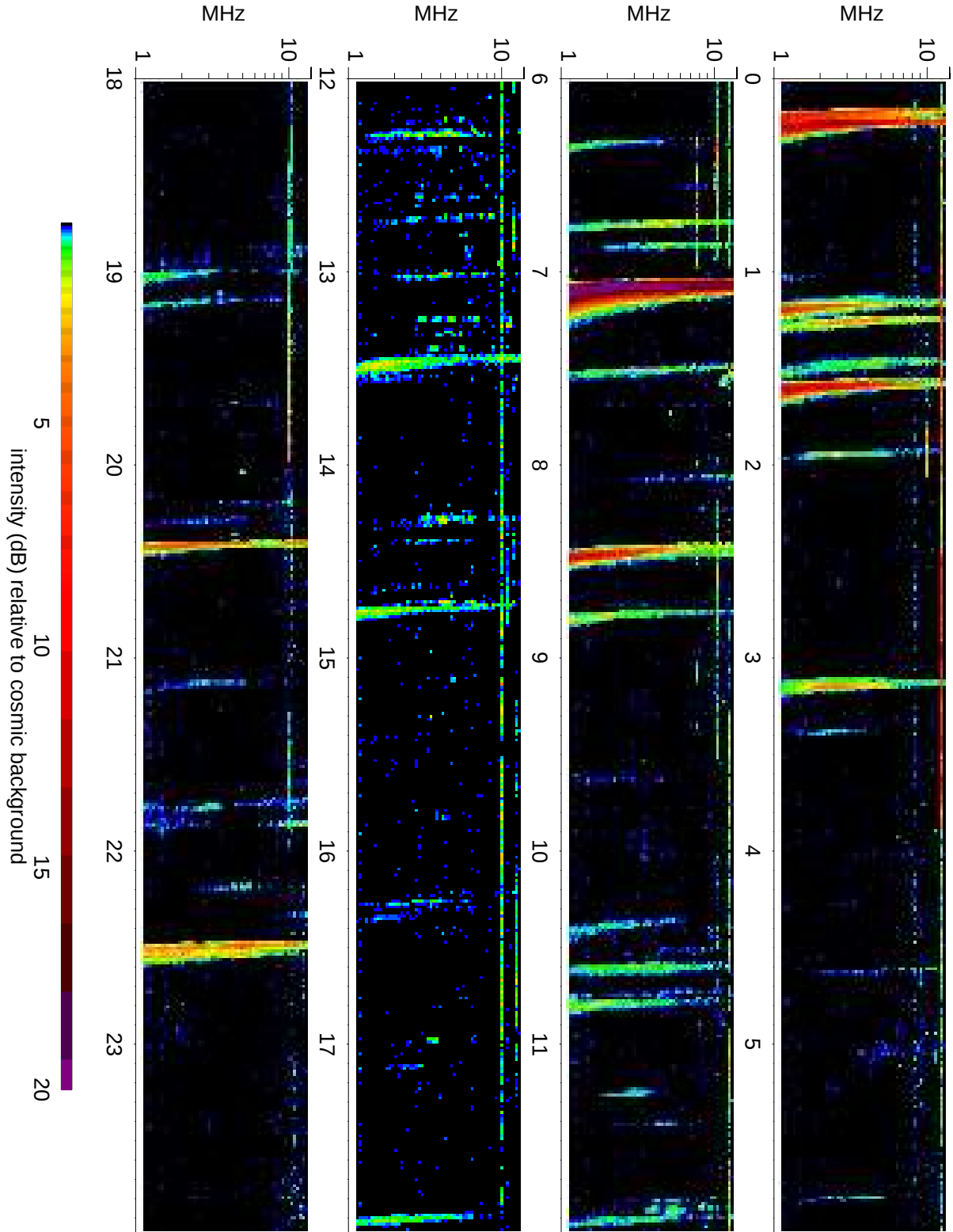
Wind Waves RAD2 receiver: 2010/02/06
