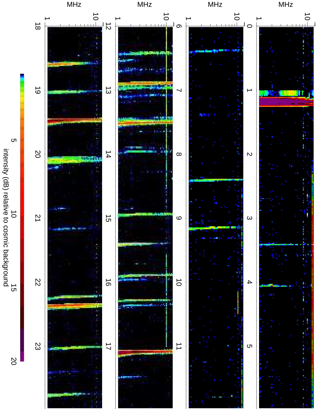
Wind Waves RAD2 receiver: 2010/02/27
