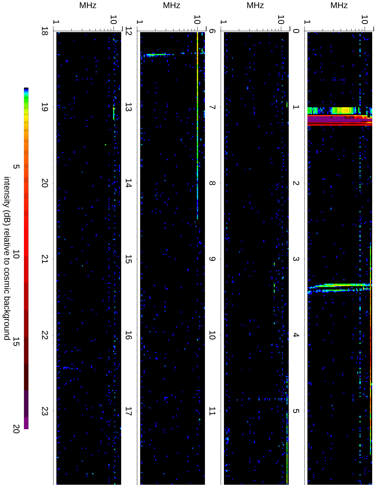
Wind Waves RAD2 receiver: 2010/03/01
