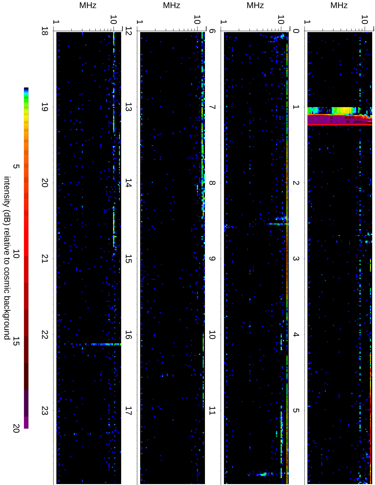
Wind Waves RAD2 receiver: 2010/03/25
