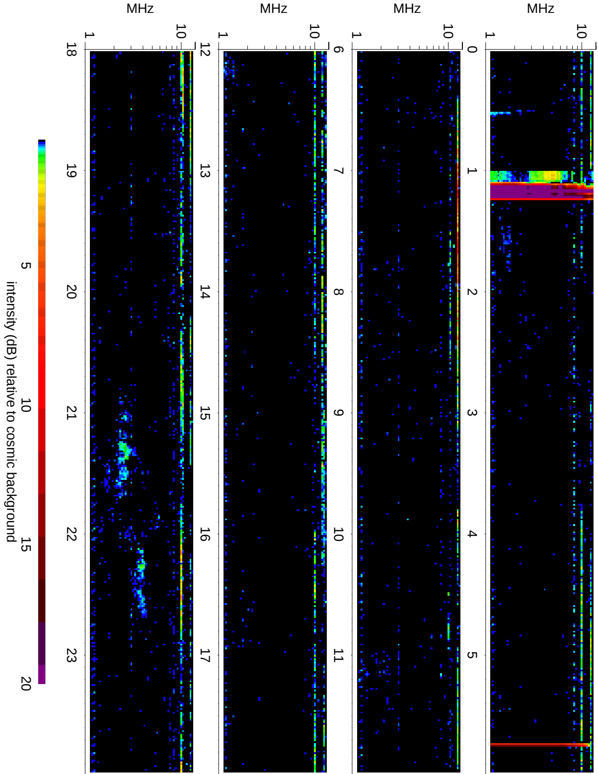
Wind Waves RAD2 receiver: 2010/04/02
