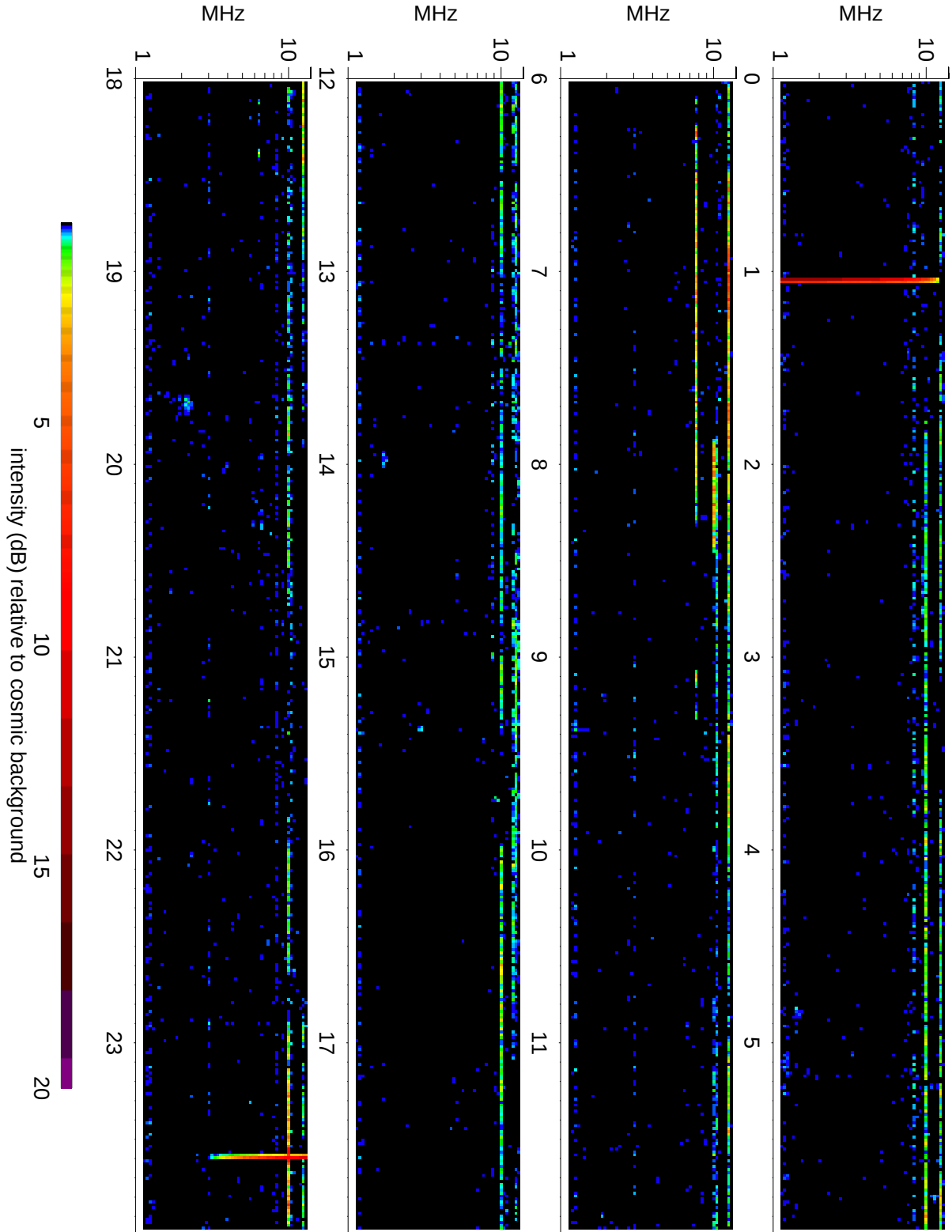
Wind Waves RAD2 receiver: 2010/04/17
