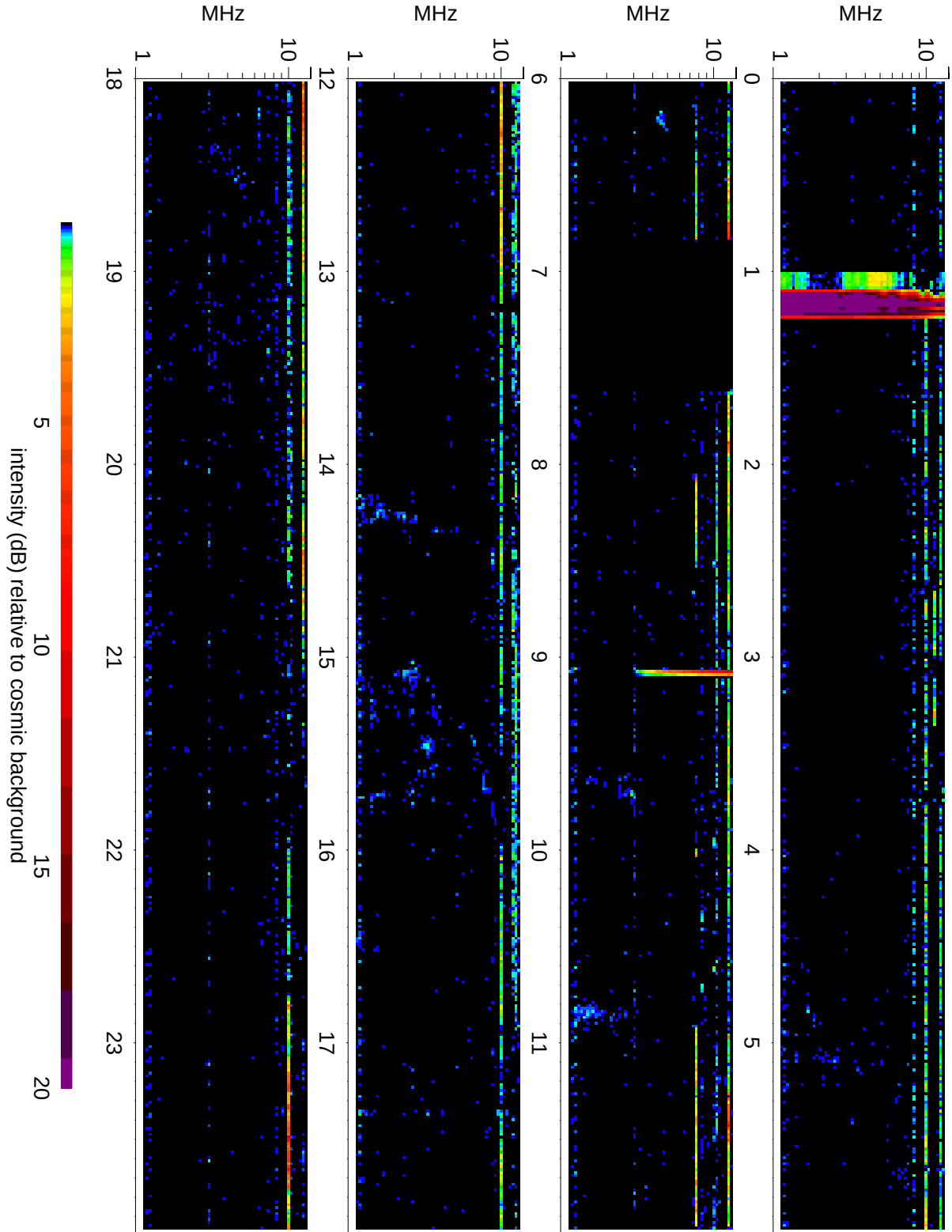
Wind Waves RAD2 receiver: 2010/04/18
