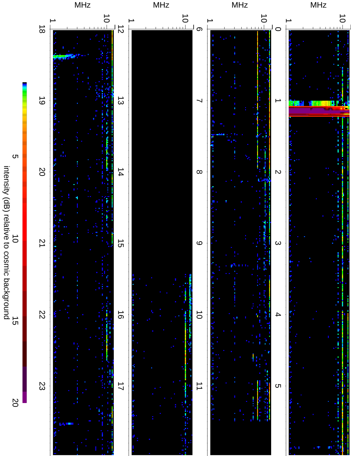
Wind Waves RAD2 receiver: 2010/05/06
