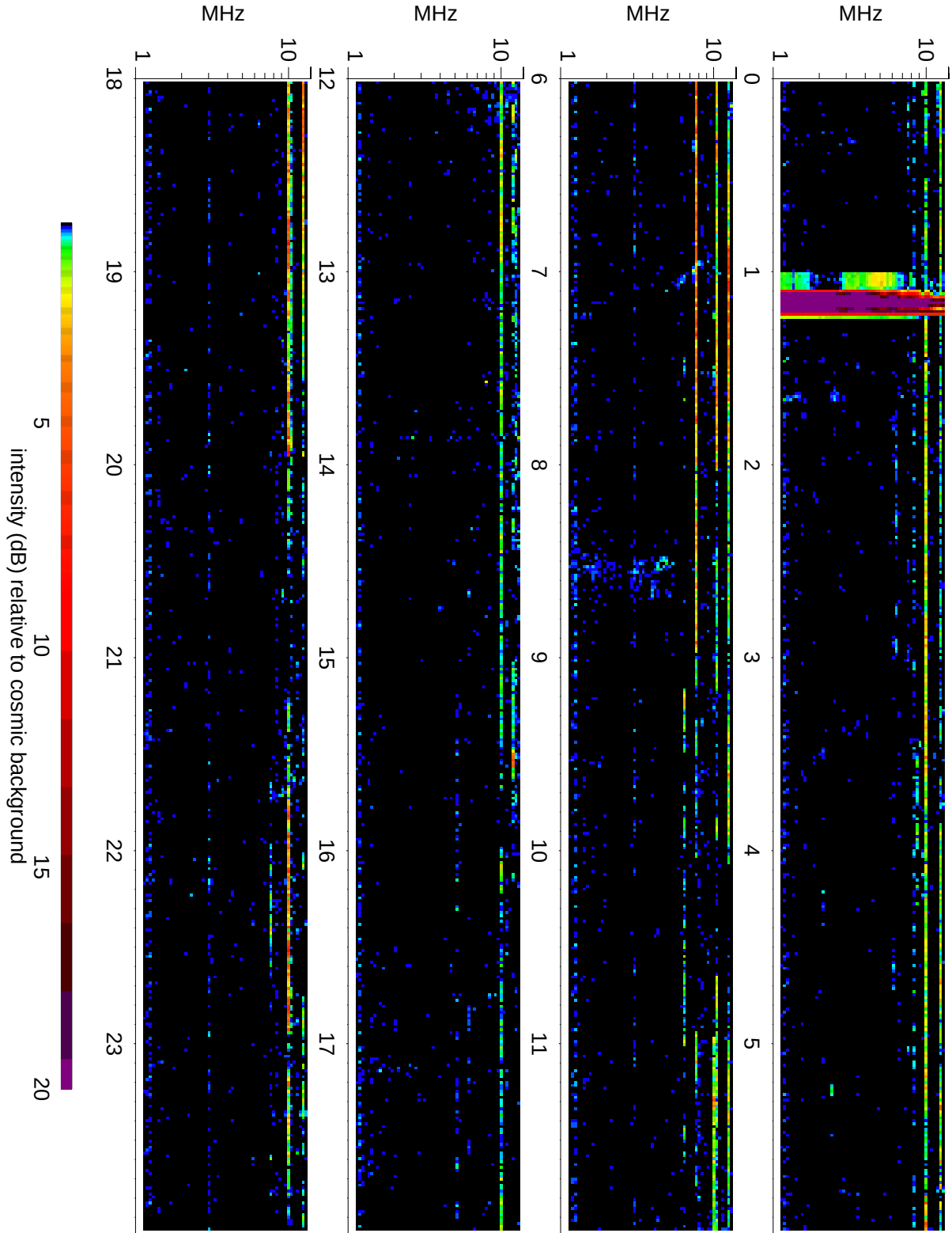
Wind Waves RAD2 receiver: 2010/05/20
