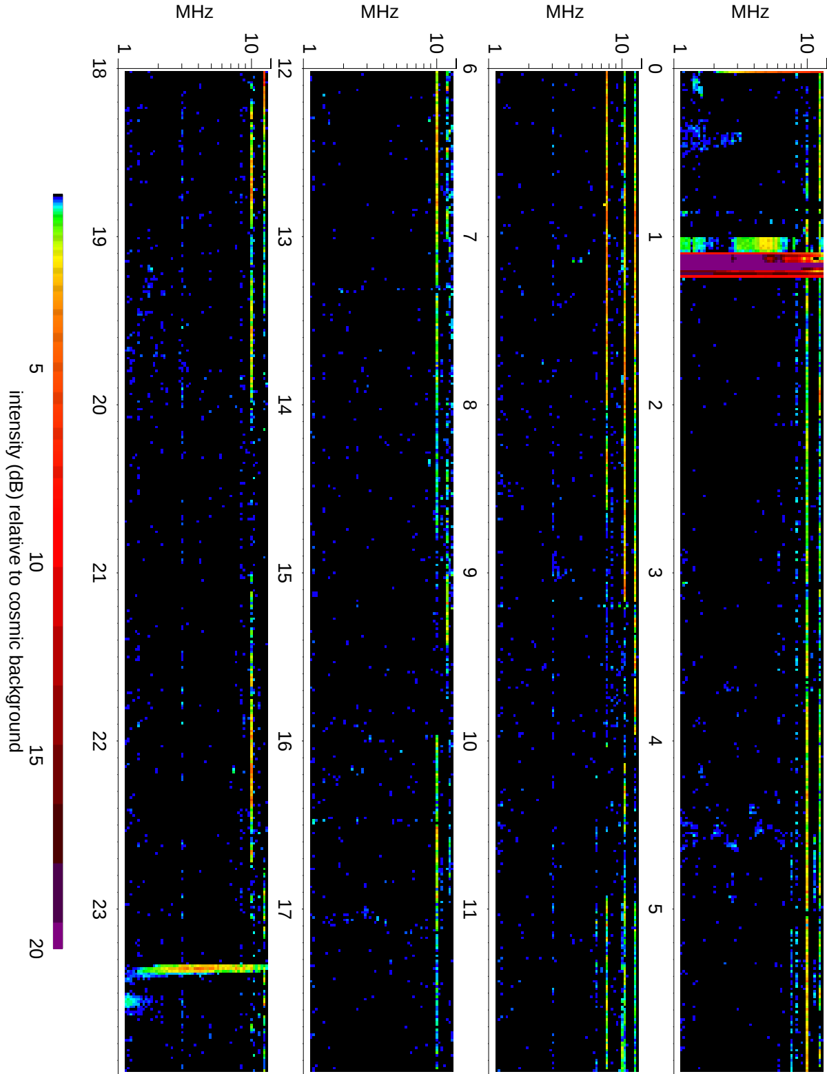
Wind Waves RAD2 receiver: 2010/05/24
